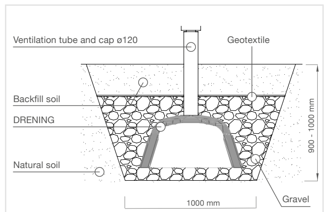
⑥ COMPLETE FILLING Cover until the ground level has been reached.
