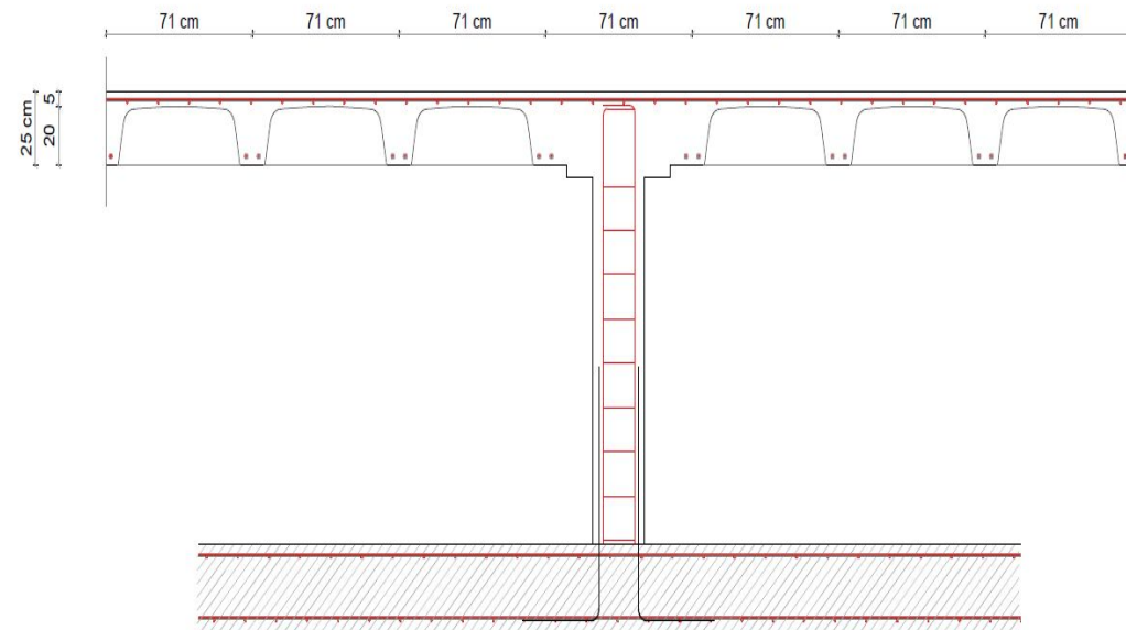
TYPOLOGICAL SECTION CONCRETE STRUCTURE
