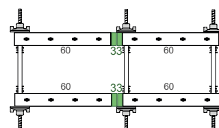
COMPENSATION 100 mm
