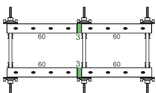
COMPENSATION 70 mm
