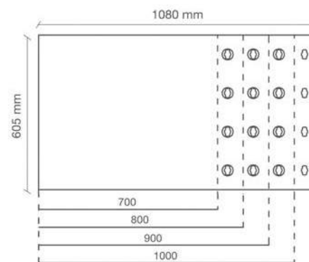
GEOPANEL STAR 70/100
