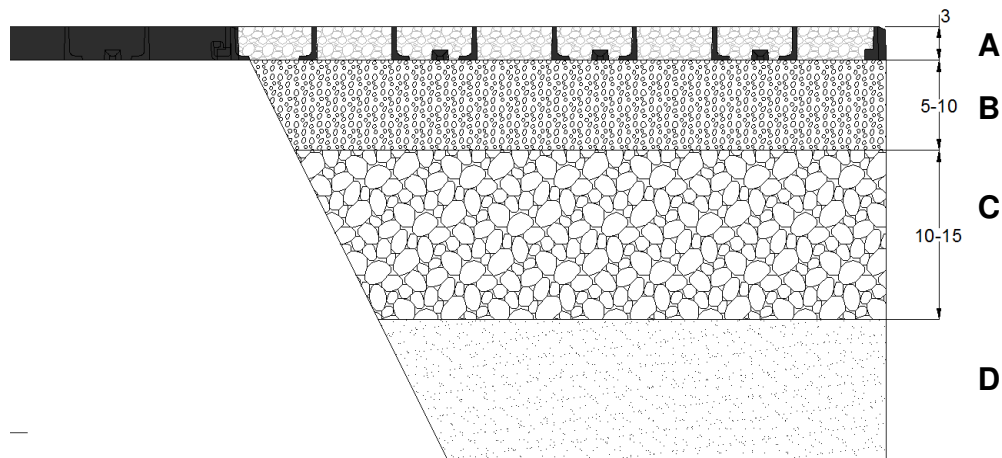
A- Runfloor S05; B- Bedding layer; C- Foundation; D- Natural soil
