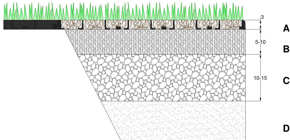
A- Runfloor S05; B- Bedding layer; C- Foundation; D- Natural soil
