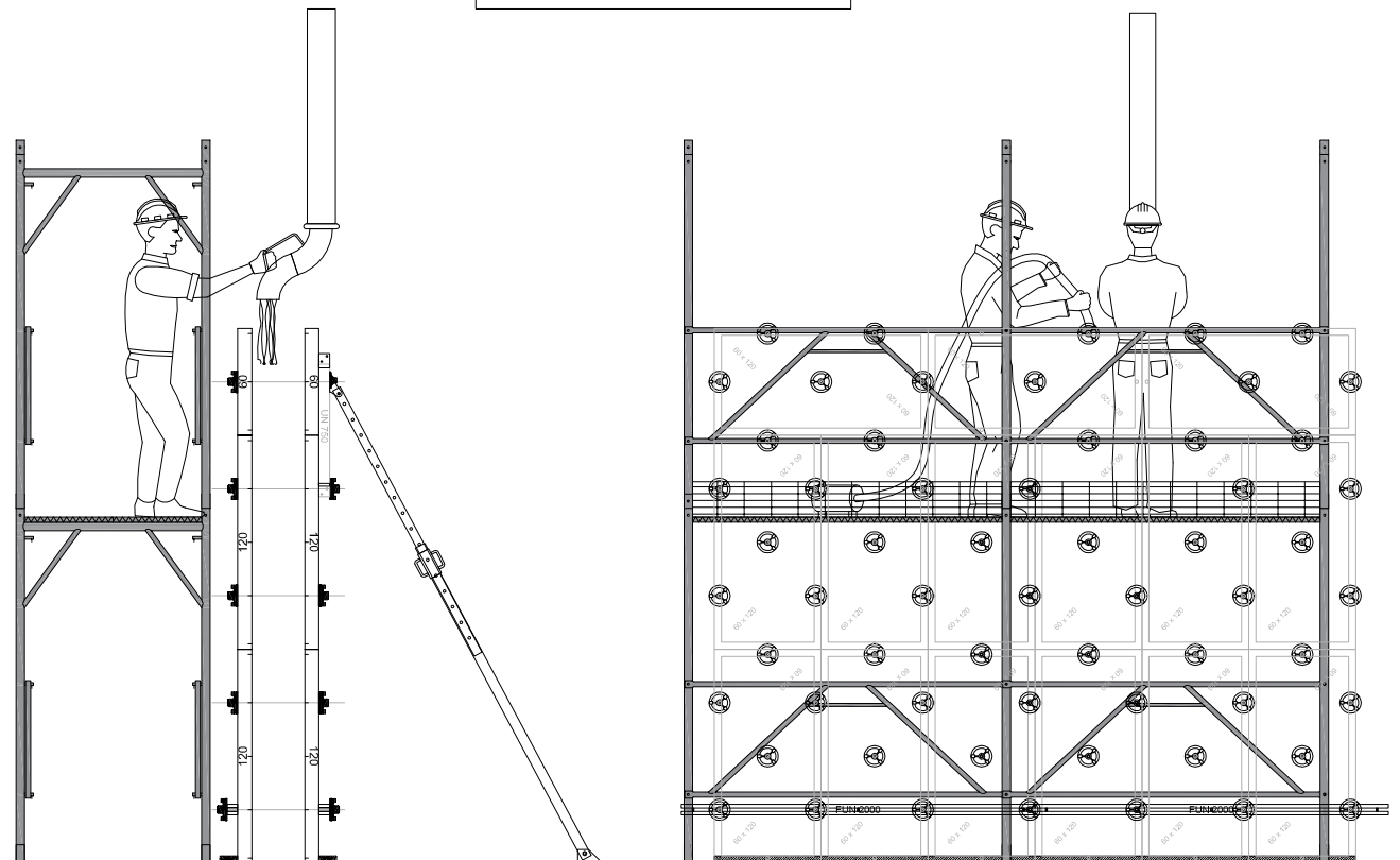
STEEL SCAFFOLDING
