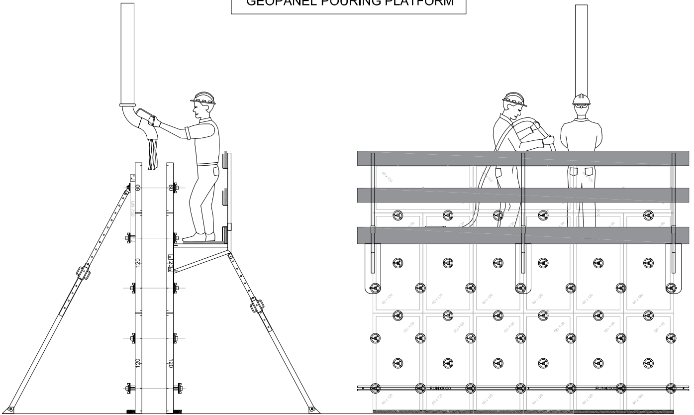
GEOPANEL POURING PLATFORM
